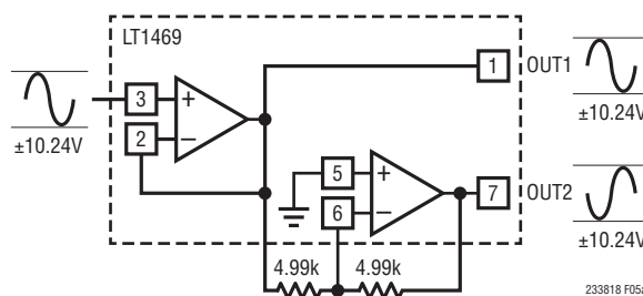
Figure 5a. LT1469 Converting a \pm 10.24\text{V} Single-Ended Signal to a \pm 20.48\text{V} Differential Input Signal
